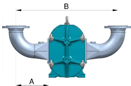
Bauform 2 90° Bogen oben in mm / inches Design 2 90° elbow up in mm / inches
