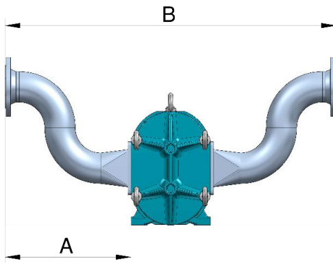
Bauform 6 Schwanenhals-Ausführung in mm Design 6 Gooseneck version in mm / inches
